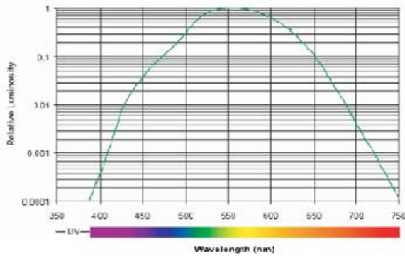
Photopic response curve
