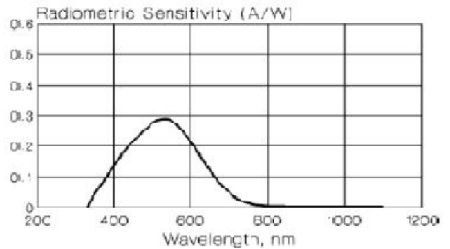
Absolute Spectral Response "B" Series (Filtered)
