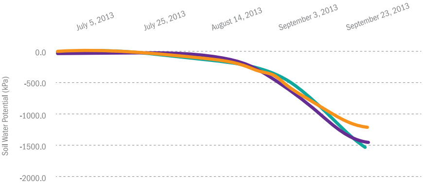
Figure 3: Time series MPS water potential data collected at 80 cm depth under a Beech forest in Switzerland. Note the excellent sensor agreement down to permanent wilting point ( -1,500 \text{ KPa} ). 3
