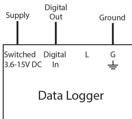
Figure 7: Wire Illustration
